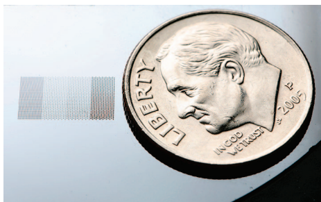
Figure 6. Mirrored pyramidal well array etched on a silicon wafer (with a U.S. dime shown for scale). The pattern on the left contains 2940 wells of three different sizes. Image courtesy of John Russell.
