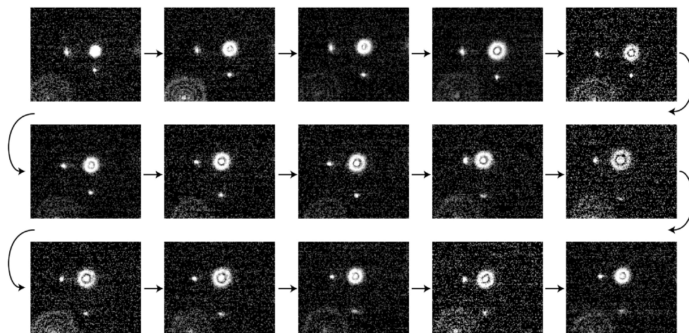
Figure 4. Higher-order maxima occur at radial positions that depend on the distance from the focal plane and appear in images as rings of light surrounding the point source. Images shown are a series from an orthogonal tracking movie of a 190 nm diameter particle in a water/glycerine solution and reproduced from McMahon et al. 1 Copyright 2009 American Chemical Society.
